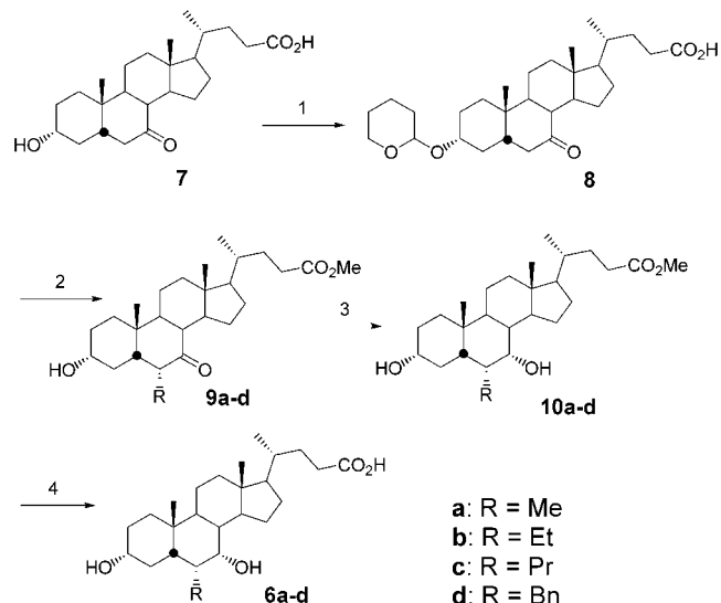
Scheme 1 a
